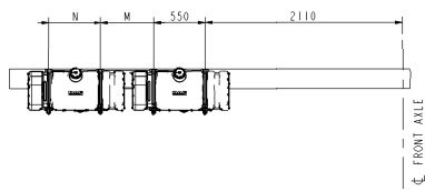
2 X 155 LITRE FUEL TANKS STANDARD POSITION
