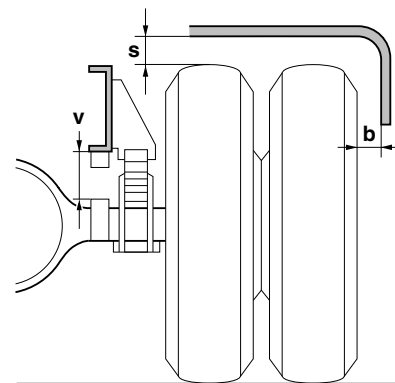
Air suspension
