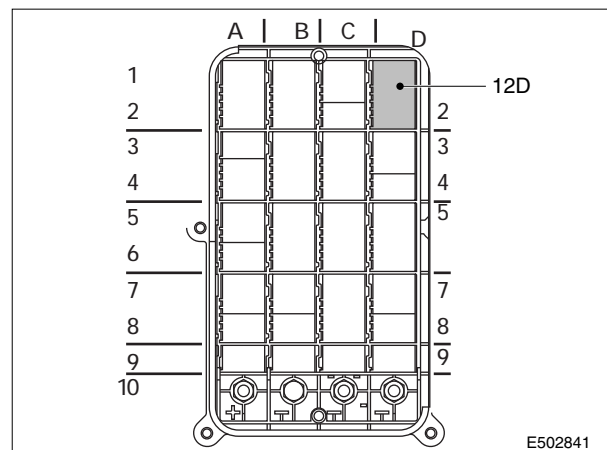
Connector 12D
