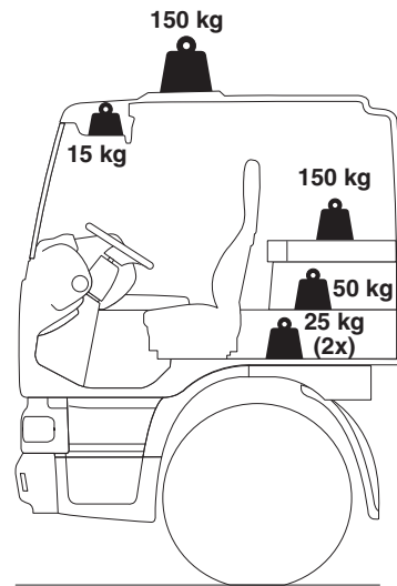
G000564 Load on cabs of CF series
