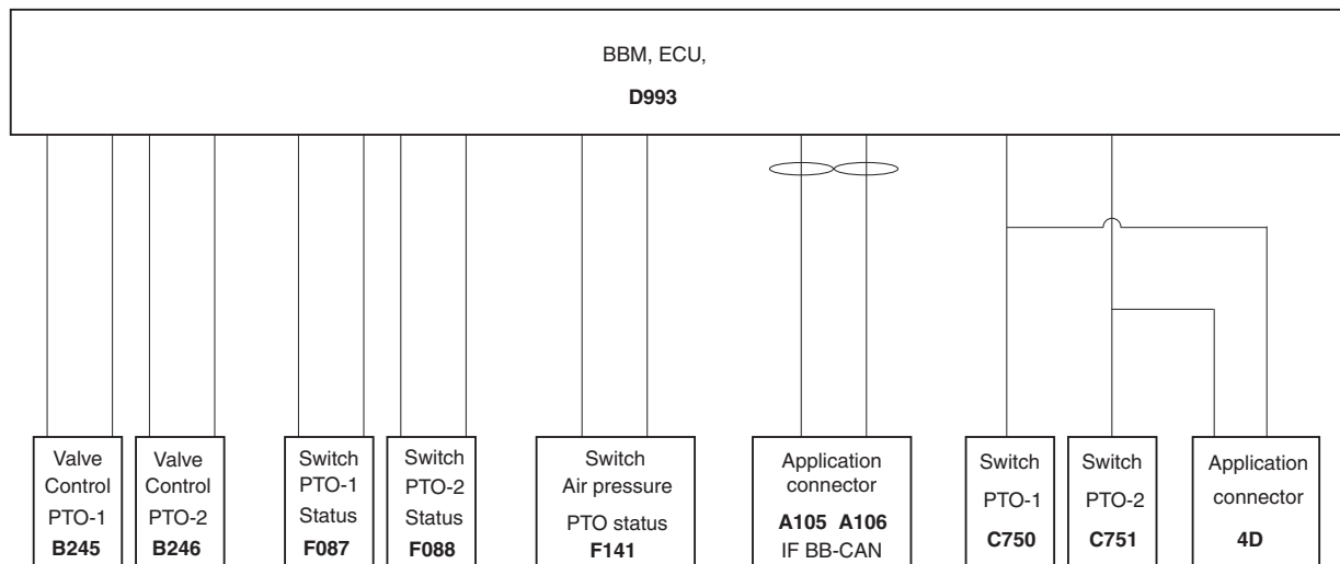
General ESC control system layout
